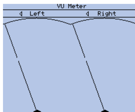
Figure 12.45.: VU-Meter
