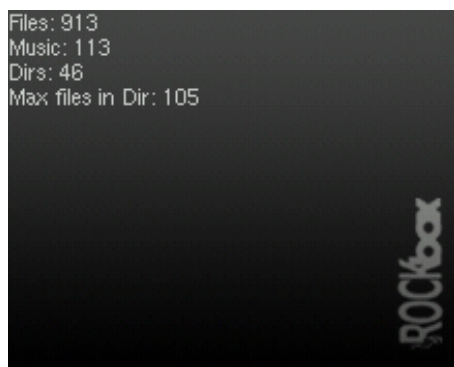
Figure 12.58.: The stats-plugin
