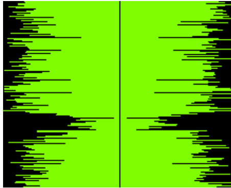
Figure 12.40.: Oscilloscope
