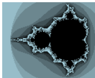
Figure 11.35.: Fractals: Mandelbrot set
