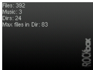
Figure 12.58.: The stats-plugin
