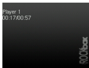
Figure 12.54.: Chess Clock
