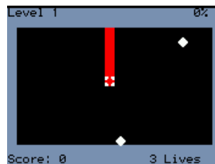
Figure 12.33.: Xbox
