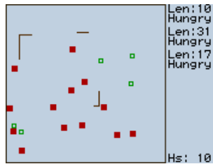
Figure 12.32.: Wormlet game
