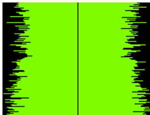
Figure 12.40.: Oscilloscope
