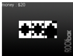
Figure 12.13.: Jackpot
