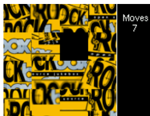
Figure 12.24.: Sliding puzzle
