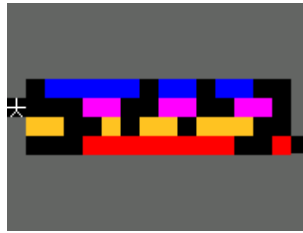
Figure 12.15.: MazezaM
