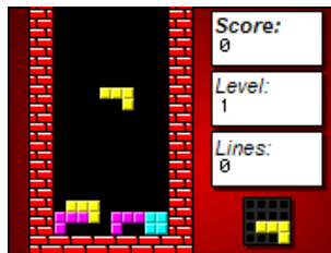
Figure 12.23.: Rockblox
