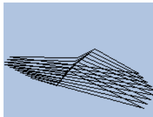
Figure 12.36.: Demystify
