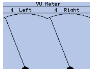
Figure 12.45.: VU-Meter
