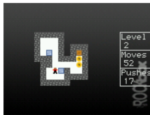
Figure 12.27.: Sokoban
