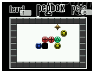
Figure 12.18.: pegbox
