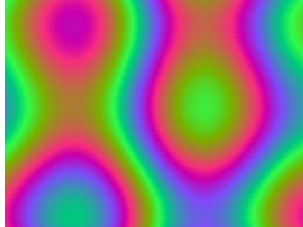
Figure 12.42.: Plasma
