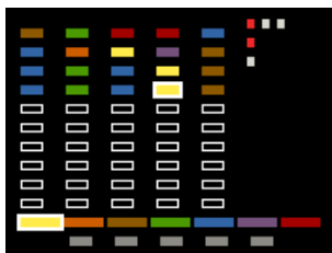
Figure 12.8.: Codebuster
