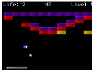
Figure 12.3.: BrickMania
