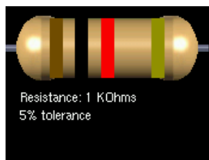
Figure 12.56.: Resistor calculator
