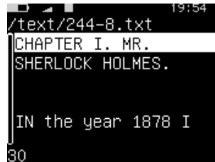
Figure 12.50.: A bookmark
