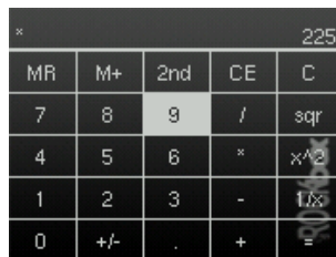
Figure 12.52.: Calculator
