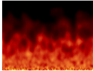
Figure 12.37.: Fire
