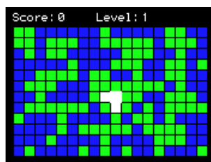
Figure 12.7.: Clix
